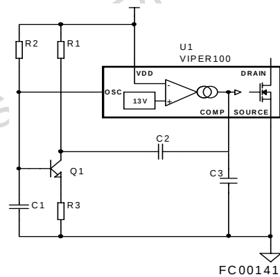
Figure 22. Slope Compensation
