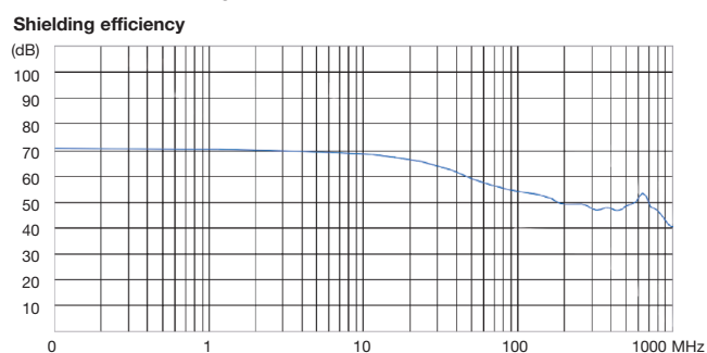
Screening Effectiveness - MHDPPK-T/M-Series
