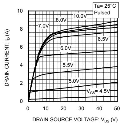
Fig.2 Typical Output Characteristics(I)
