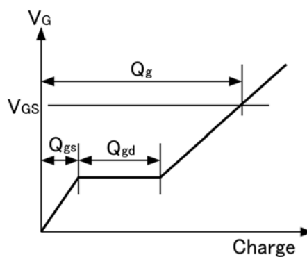
Fig.2-2 Gate charge waveform
