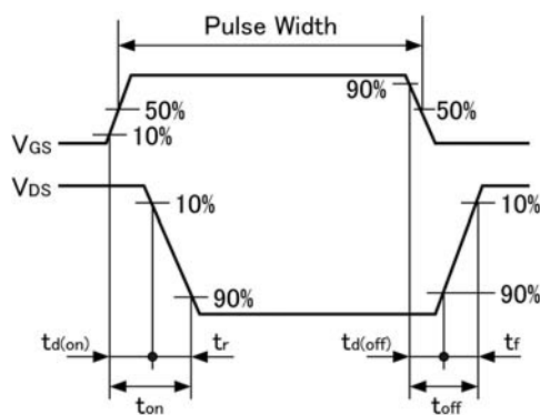
Fig.1-2 Switching waveforms
