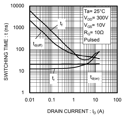
Fig.14 Switching Characteristics
