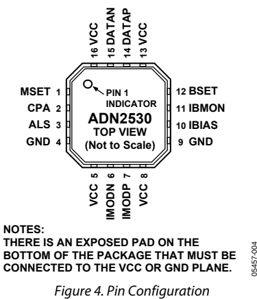
Figure 4. Pin Configuration
