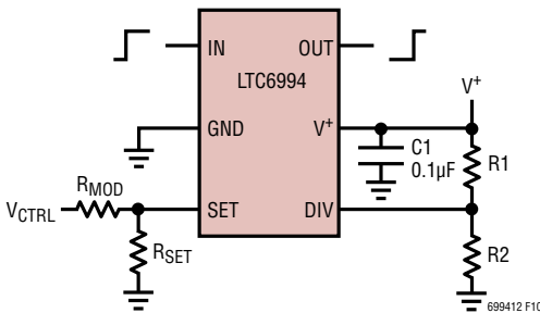
Figure 10. Voltage-Controlled Delay
