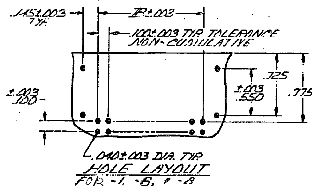
HOLE LAYOUT
