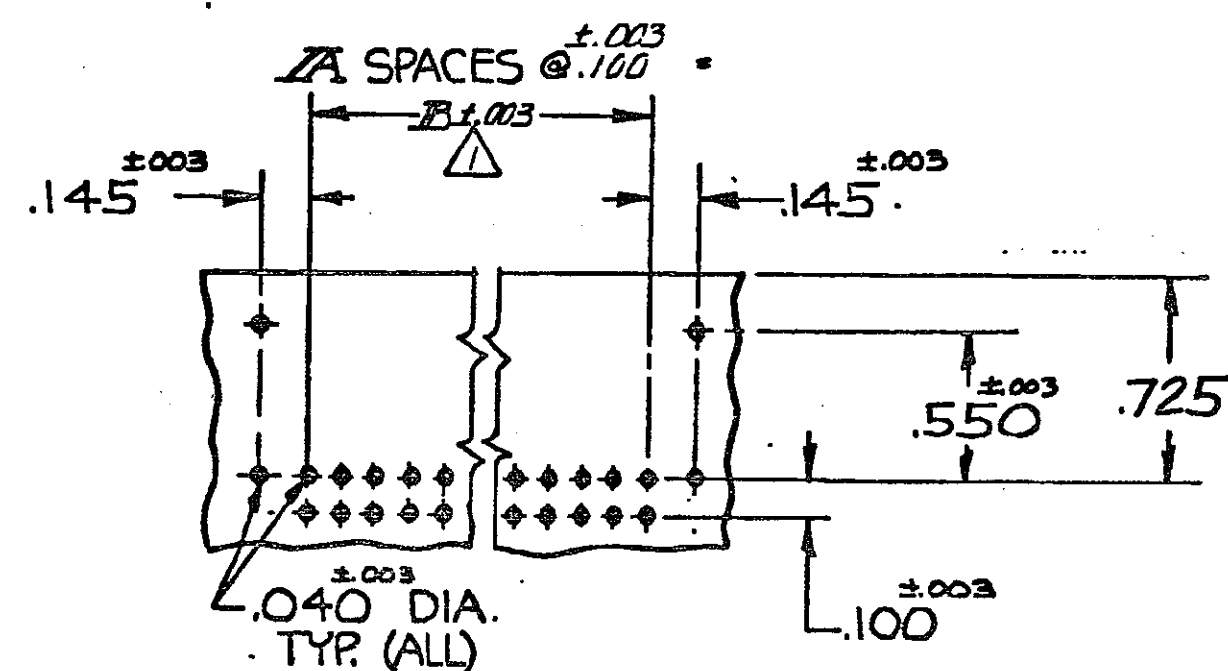
HOLE LAYOUT
