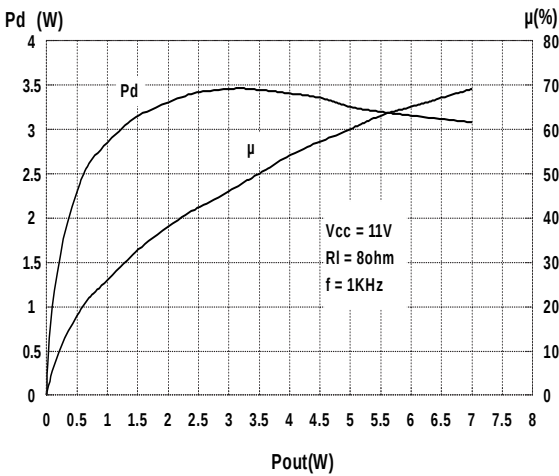
Figure 9: Total Power Dissipation & Efficiency vs. Output Power
