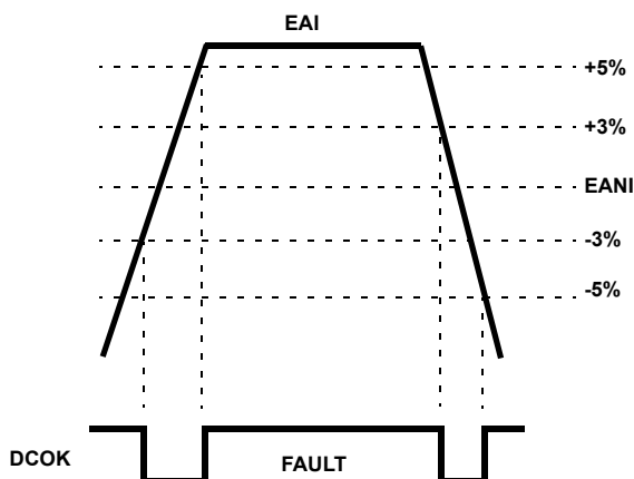
FIGURE 14. UNDERVOLTAGE-OVERVOLTAGE WINDOW
