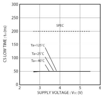
Fig.17 CS low time tCS
