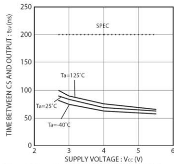
Fig.24 Time from CS to output establishment tSV
