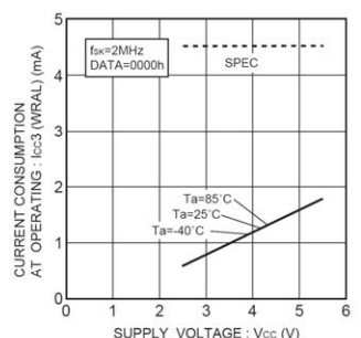
Fig.14 Consumption current at WRAL action I_{CC3}(\text{WRAL}, f_{SK}=2\text{MHz})
