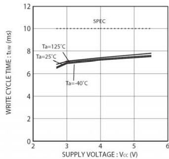
Fig.26 Write cycle time tE/W
