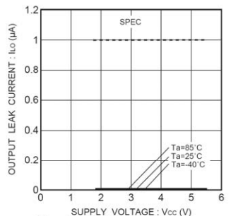
Fig.11 Output leak current I_{LO}(\text{DO})
