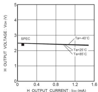
Fig.8 H output voltage V_{OH-IOH}(V_{CC}=2.5\text{V})
