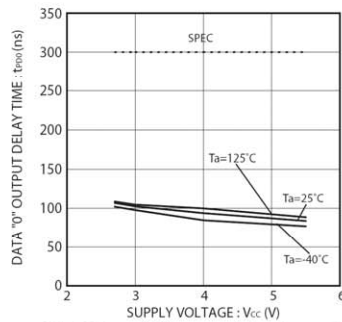
Fig.23 Data "0" output delay time tPD0
