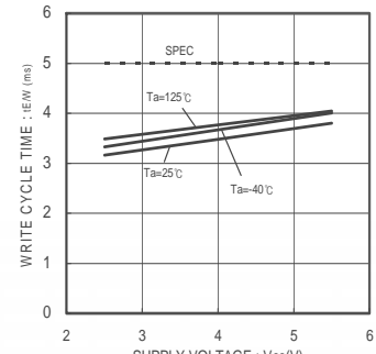
Fig.26-1 Write cycle time tE/W
