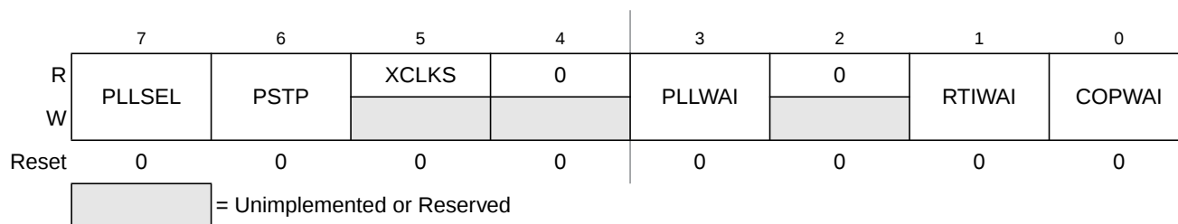
Figure 8-8. S12XECRG Clock Select Register (CLKSEL)
