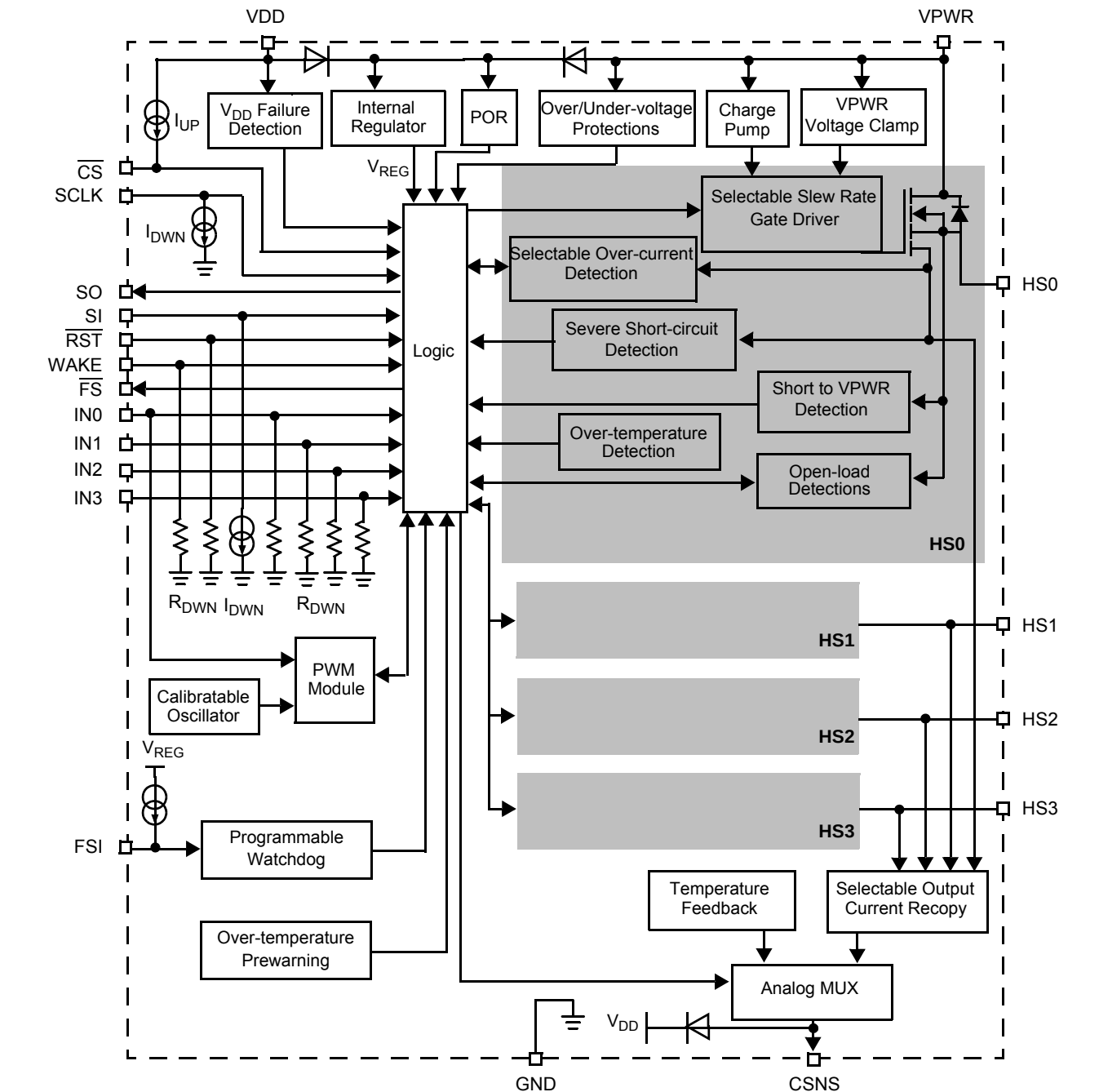
Figure 2. 15XS3400 Simplified Internal Block Diagram
