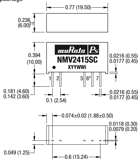
SIP package
