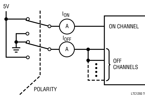
On and Off Channel Leakage Current
