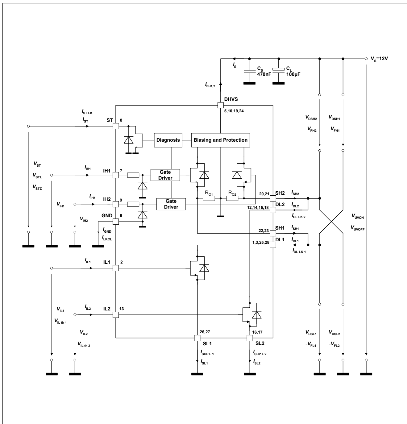
Figure 2 Terms BTM7700G
