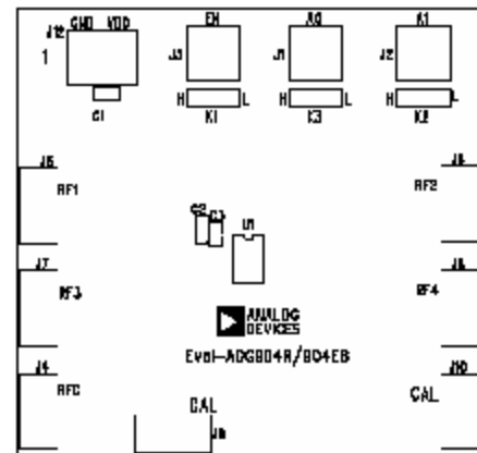
Figure 30. ADG904/ADG904-R Evaluation Board Top View
