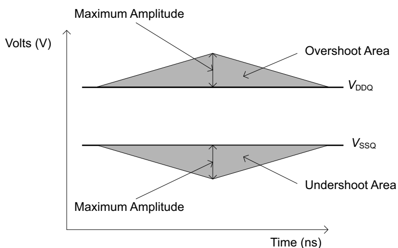
FIGURE 7 AC Overshoot / Undershoot Diagram for Clock, Data, Strobe and Mask Pins
