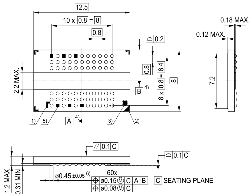
FIGURE 11 Package Outline P-TFBGA-60
