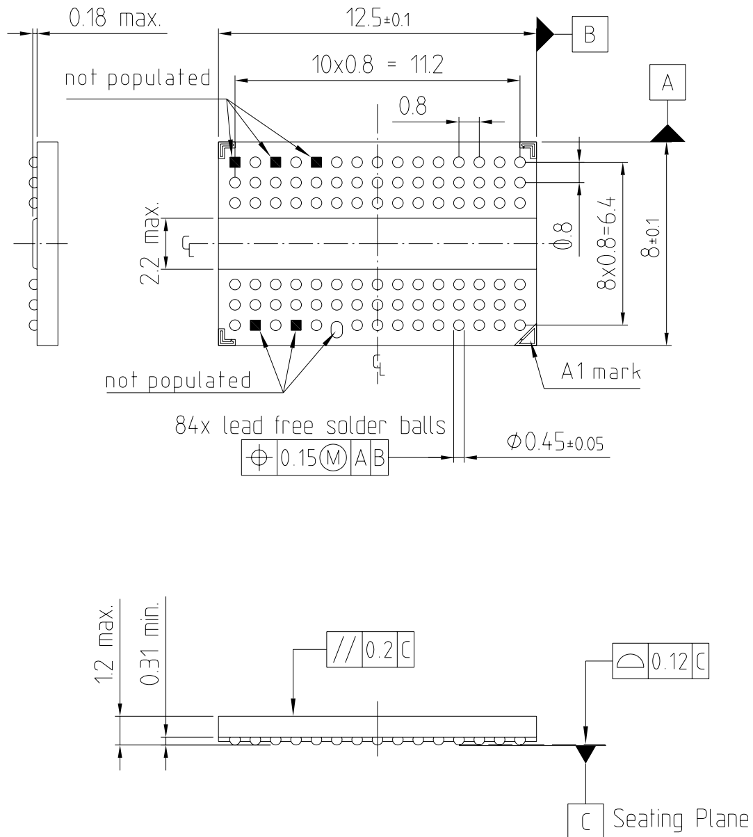
FIGURE 16 Package Outline PG-TFBGA-84
