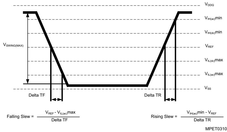
FIGURE 4 Single-ended AC Input Test Conditions Diagram
