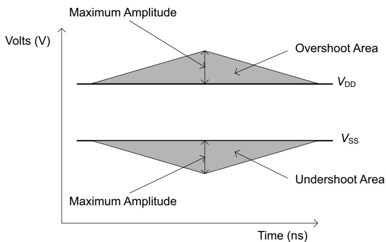
FIGURE 6 AC Overshoot / Undershoot Diagram for Address and Control Pins
