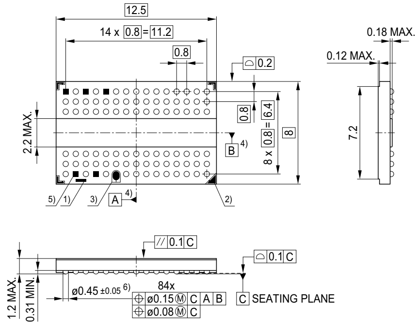
FIGURE 14 Package Outline P-TFBGA-84
