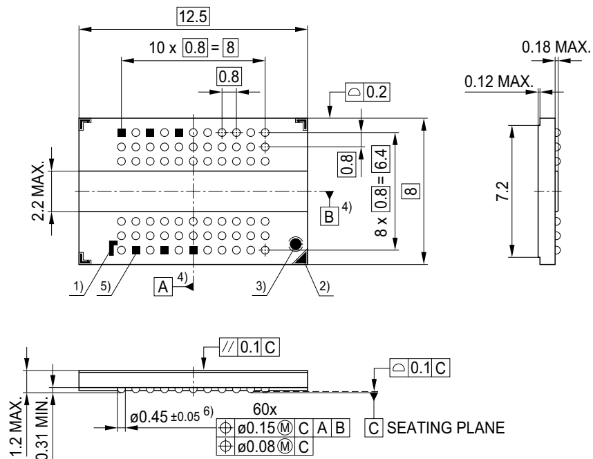
FIGURE 12 Package Outline PG-TFBGA-60
