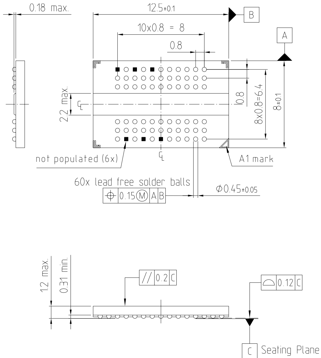
FIGURE 13 Package Outline PG-TFBGA-60
