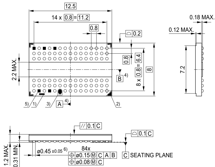
FIGURE 15 Package Outline PG-TFBGA-84
