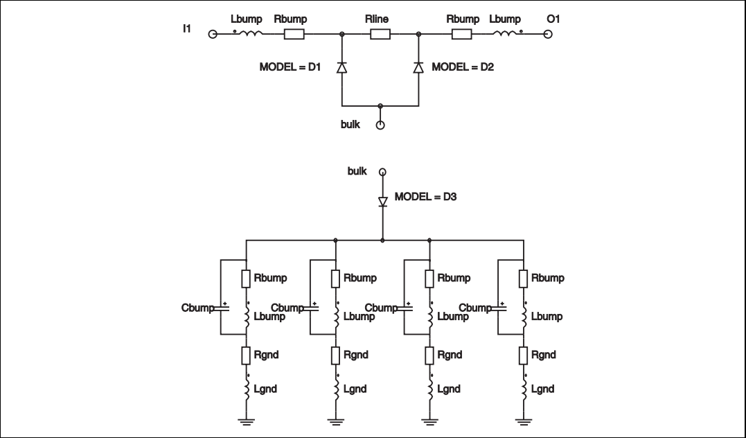
Figure 8. Aplac model
