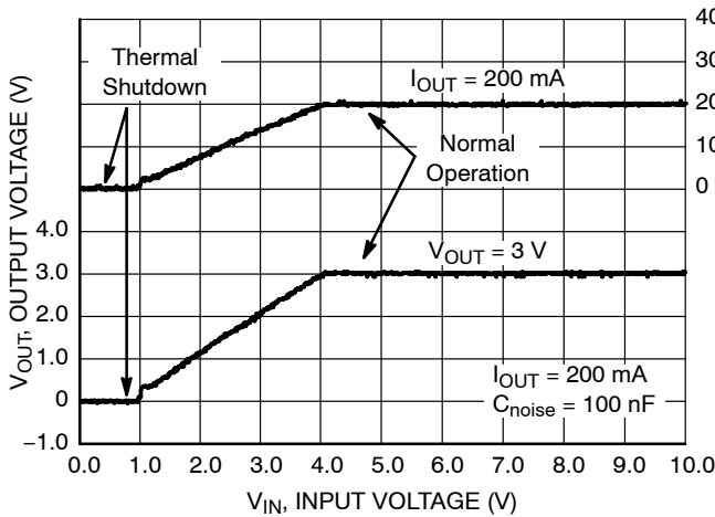
Figure 43. Thermal Shutdown Protection V_{OUT} = 3\text{ V} , C_{noise} = 100\text{ nF} , C_{OUT} = 1\text{ }\mu\text{F}
