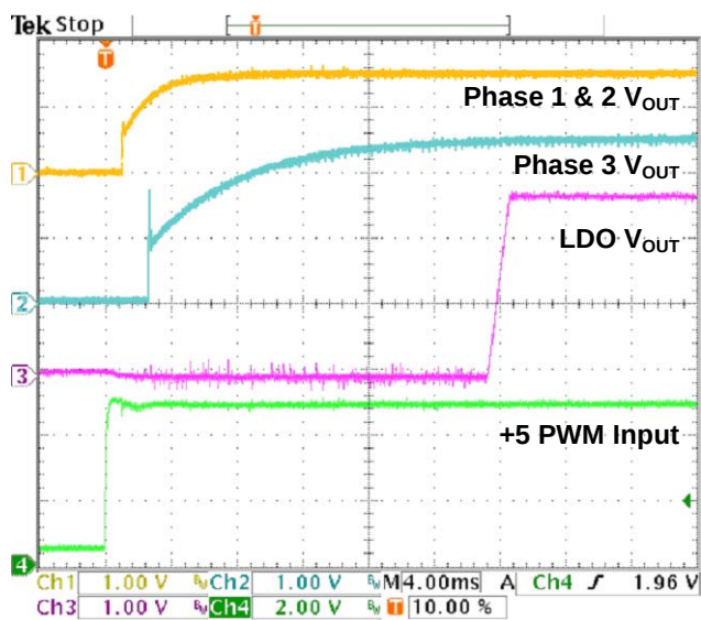
Figure 5 – Start-Up Sequence
