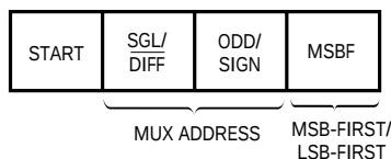
LTC1091 DATA INPUT ( D_{IN} ) WORD:
