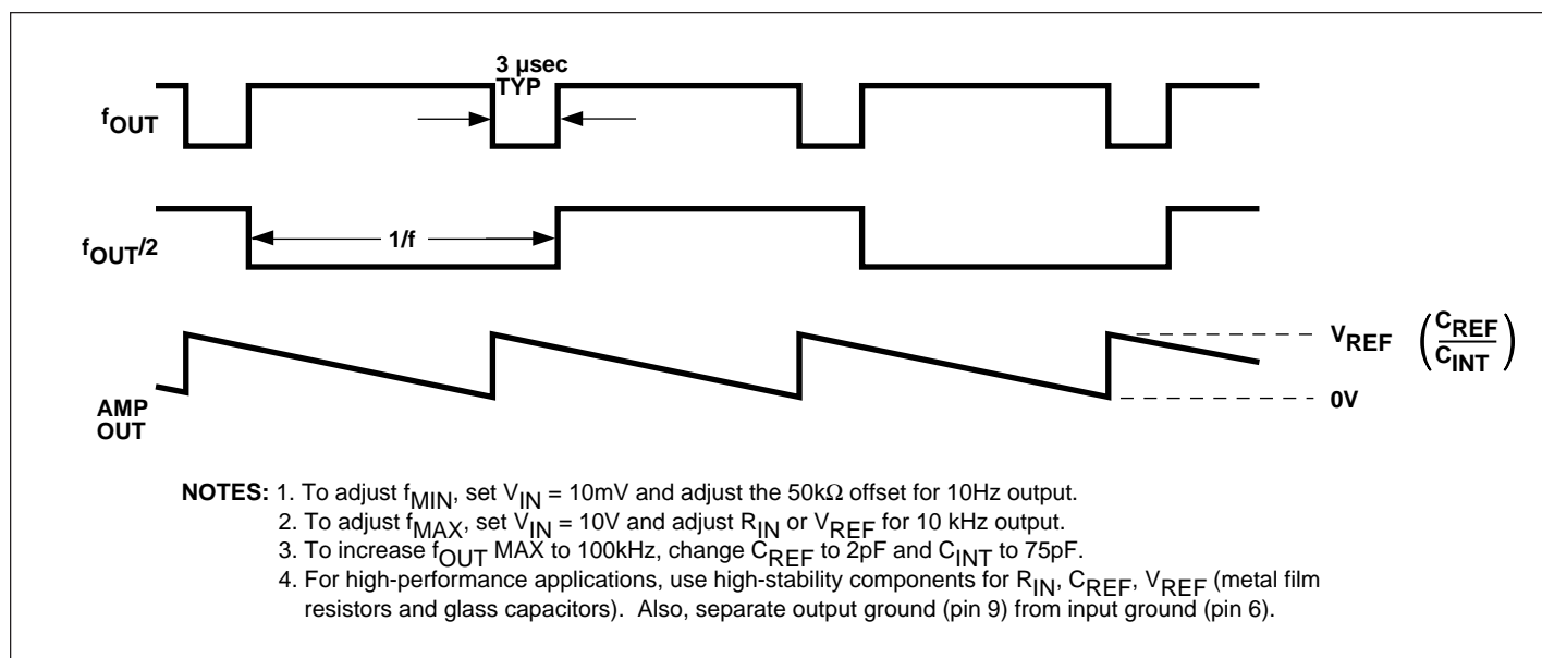
Figure 2 . Output Waveforms
