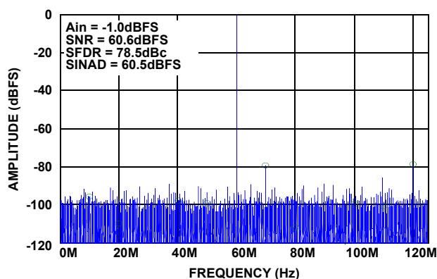
FIGURE 17. SINGLE-TONE SPECTRUM @ 190MHz
