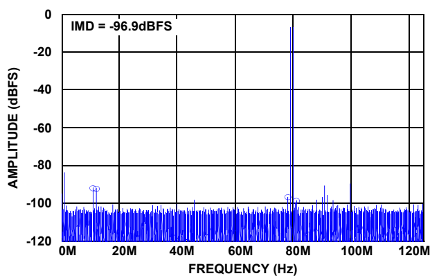
FIGURE 21. TWO-TONE SPECTRUM @ 170MHz
