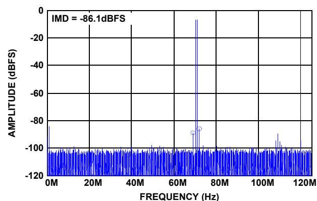
FIGURE 20. TWO-TONE SPECTRUM @ 70MHz
