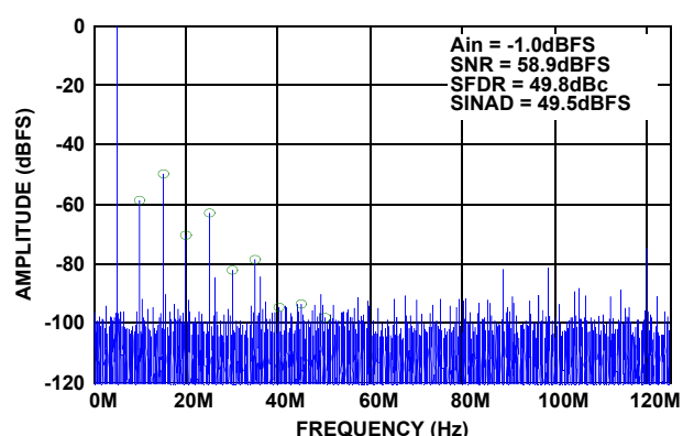
FIGURE 19. SINGLE-TONE SPECTRUM @ 995MHz
