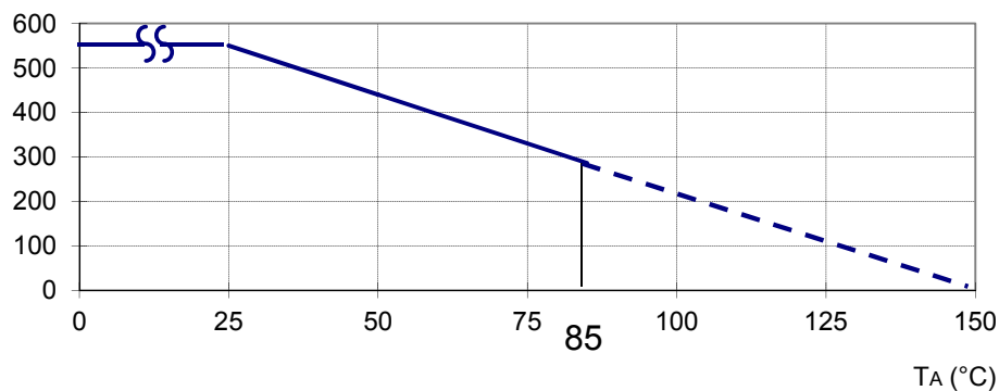
Power Dissipation Curve
