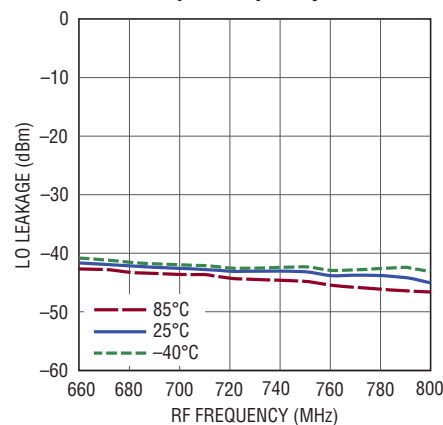
LO-RF Leakage vs RF Output Frequency
