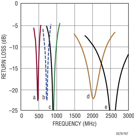
Figure 7. RF Output Return Loss with 450MHz (a), 740MHz (b), 900MHz (c), 1950MHz (d) and 2600MHz (e) Matching
