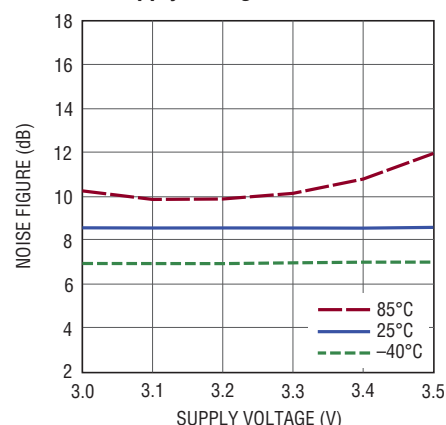
SSB Noise Figure vs Supply Voltage
