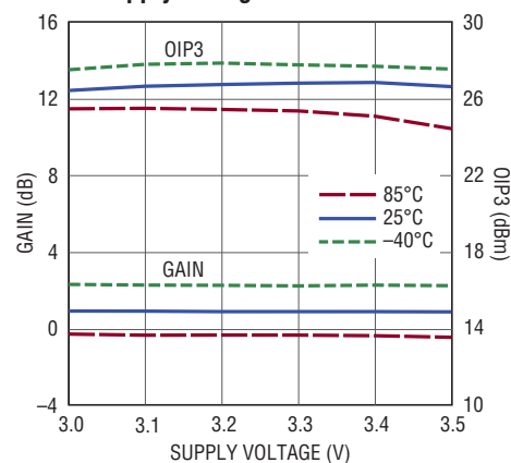
Conversion Gain and OIP3 vs Supply Voltage
