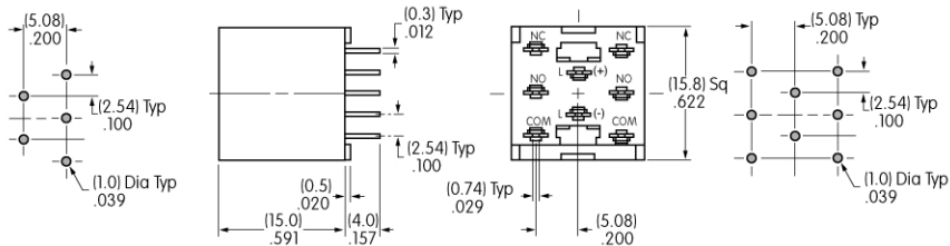
AT712 Double Pole • Straight PC Terminals
