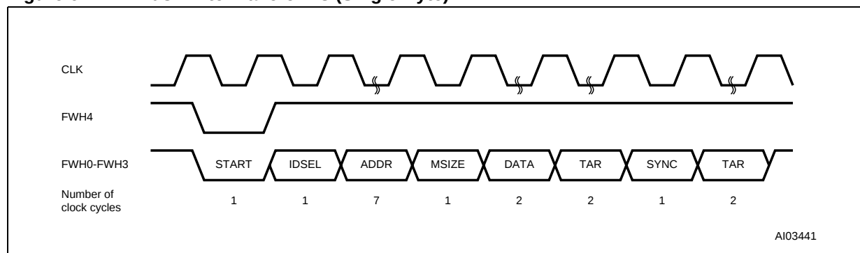
Figure 6. FWH Bus Write Waveforms (Single Byte)
