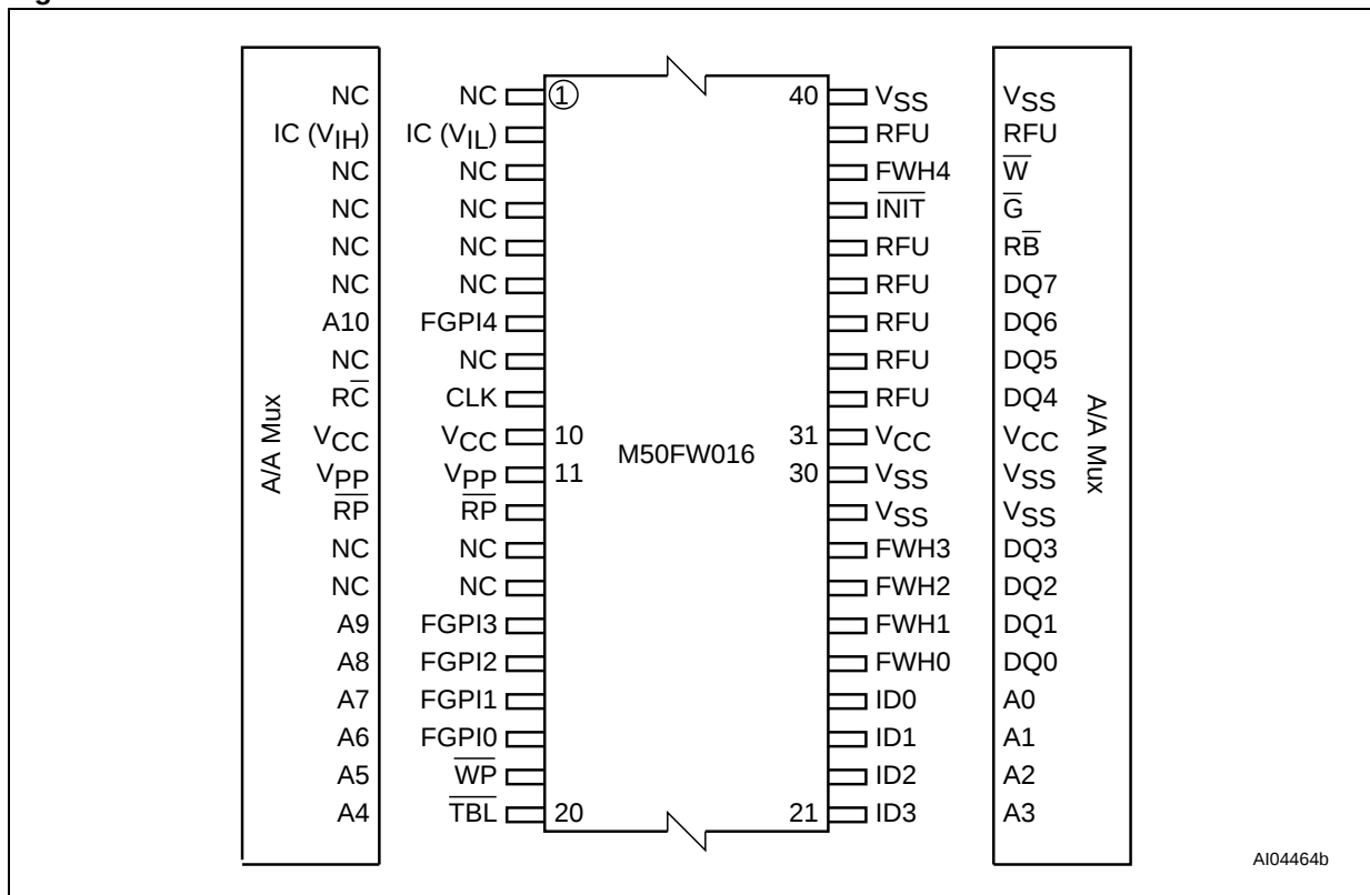
Figure 4. TSOP Connections
