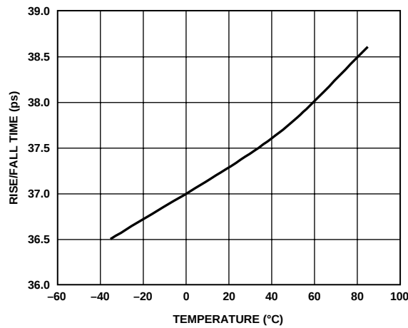
Figure 6. Rise/Fall Time vs. Temperature
