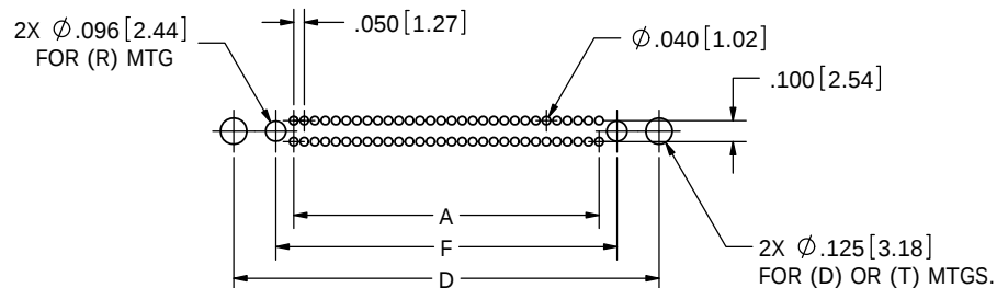
PCB LAYOUT, CONNECTOR SIDE
