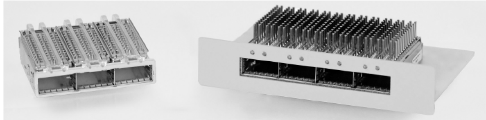
Through Bezel
