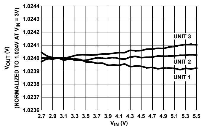
FIGURE 4. LINE REGULATION, 3 UNITS
