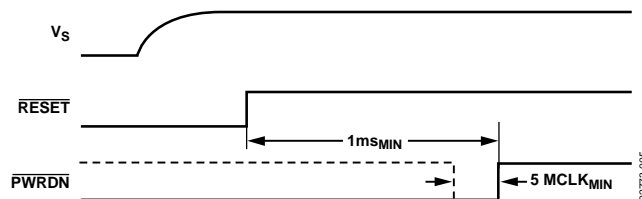
Figure 5. Power-Up Sequence for Tx Data Path
