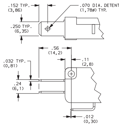
4A .250" QUICK CONNECT
