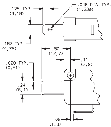
40 .187" QUICK CONNECT
