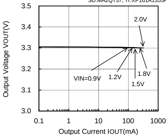
XC9104D091MR (PWM/PFM,100kHz,3.3V)
