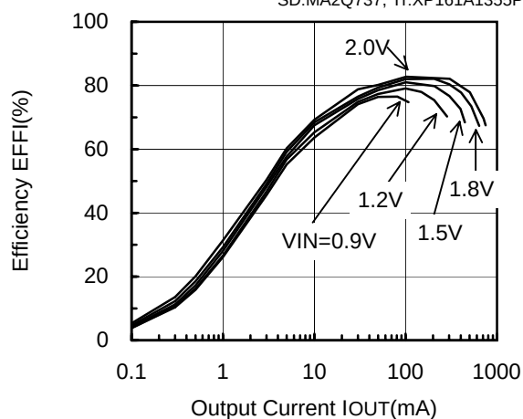
XC9103D093MR (PWM,300kHz,3.3V)
