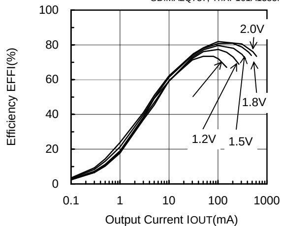
XC9103D095MR (PWM,500kHz,3.3V)
