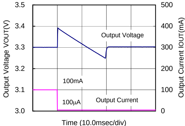
XC9103D093MR(PWM,300kHz,3.3V)
