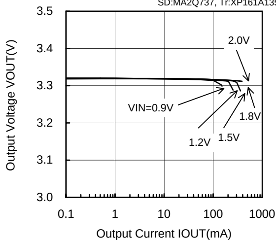
XC9104D092MR (PWM/PFM,180kHz,3.3V)
