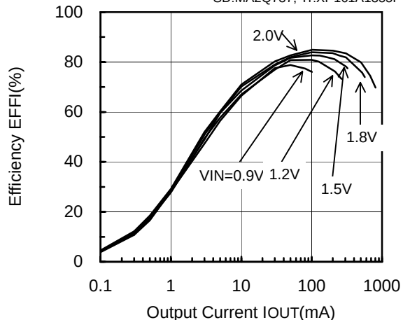
XC9103D093MR (PWM,300kHz,3.3V)
