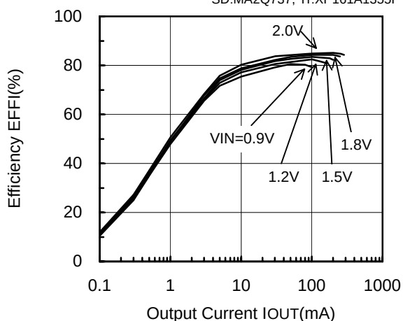
XC9103D091MR (PWM,100kHz,3.3V)
