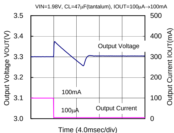
XC9103D092MR(PWM,180kHz,3.3V)
