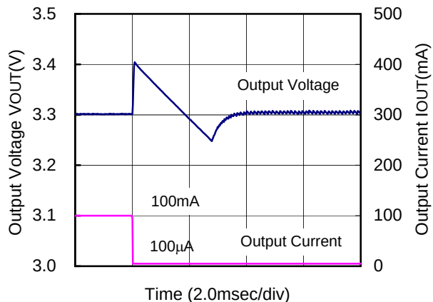
XC9104D092MR(PWM/PFM,180kHz,3.3V)
