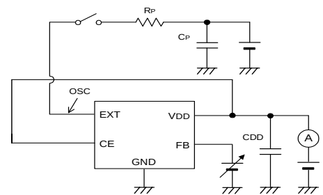
CIRCUIT ④
