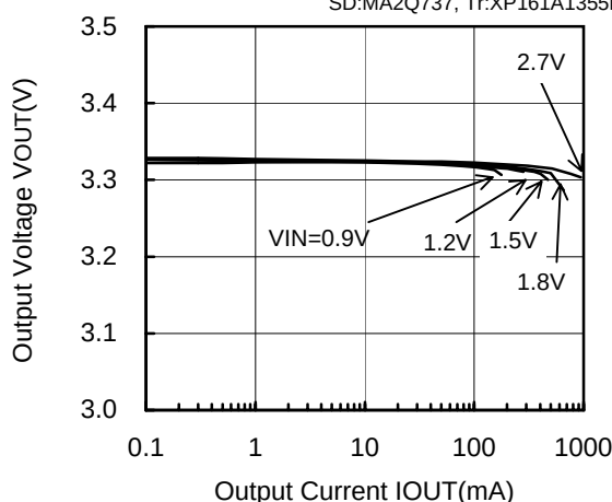
XC9104D093MR (PWM/PFM,300kHz,3.3V)
