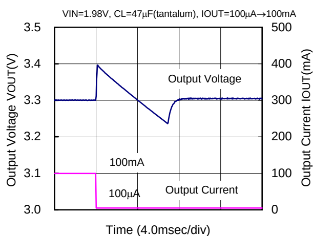
XC9104D092MR(PWM/PFM,180kHz,3.3V)
