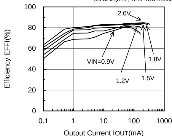
XC9104D091MR (PWM/PFM,100kHz,3.3V)
