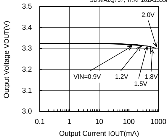
XC9104D093MR (PWM/PFM,300kHz,3.3V)
