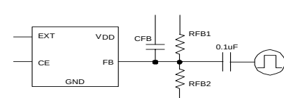
CIRCUIT ⑥
