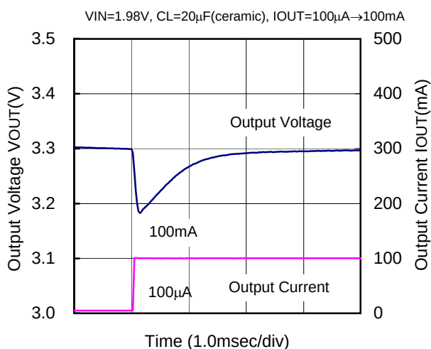
XC9104D093MR(PWM/PFM,300kHz,3.3V)
