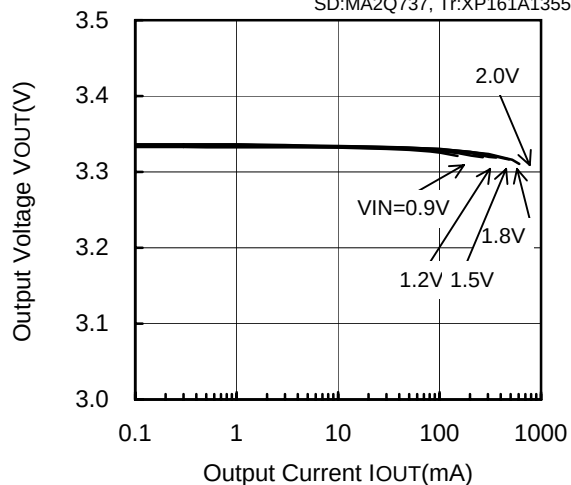
XC9103D095MR (PWM,500kHz,3.3V)
