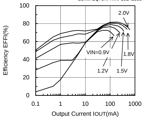
XC9104D095MR (PWM/PFM,500kHz,3.3V)
