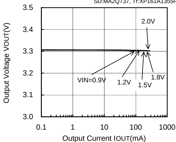
XC9103D091MR (PWM,100kHz,3.3V)
