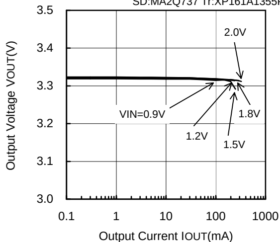
XC9103D092MR (PWM,180kHz,3.3V)
