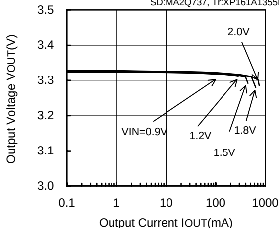
XC9103D093MR (PWM,300kHz,3.3V)
