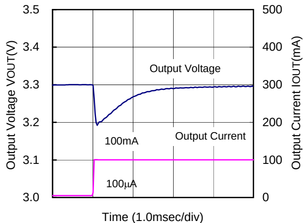
XC9103D092MR(PWM,180kHz,3.3V)
