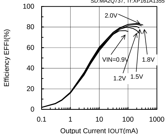
XC9103D092MR (PWM,180kHz,3.3V)
