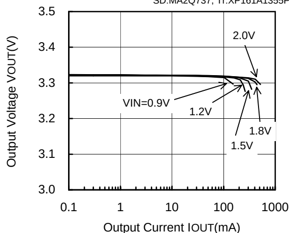
XC9104D092MR (PWM/PFM,180kHz,3.3V)
