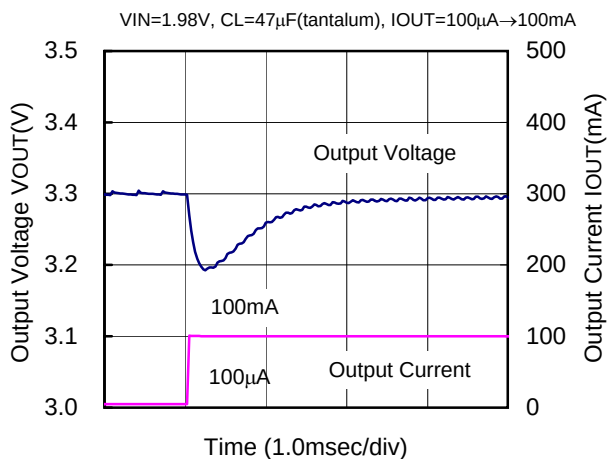
XC9104D092MR(PWM/PFM,180kHz,3.3V)
