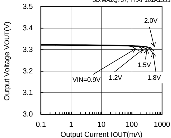
XC9103D092MR (PWM,180kHz,3.3V)
