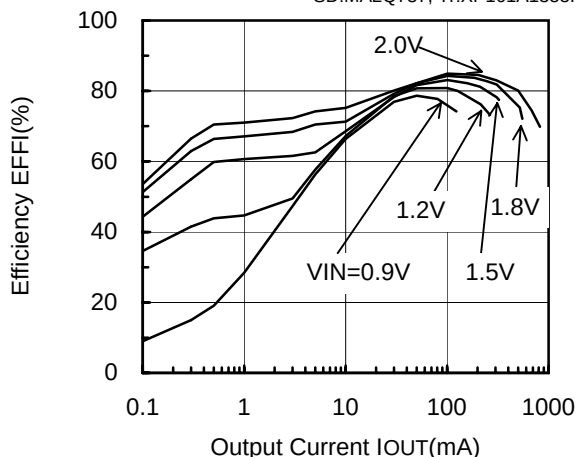
XC9104D093MR (PWM/PFM,300kHz,3.3V)
