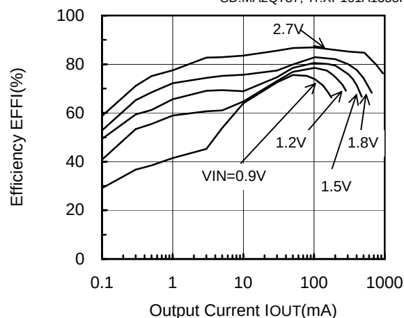
XC9104D093MR (PWM/PFM,300kHz,3.3V)
