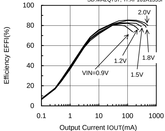
XC9103D092MR (PWM,180kHz,3.3V)
