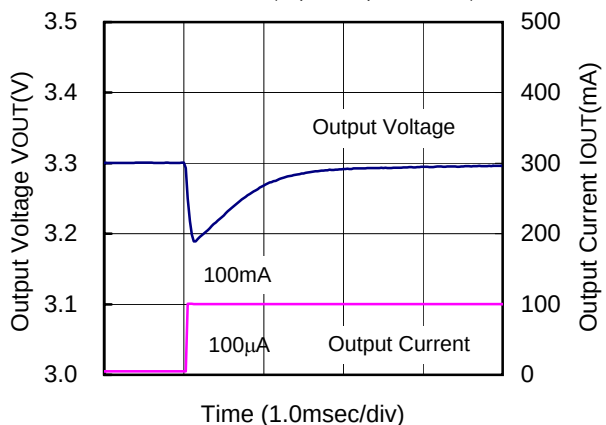
XC9103D093MR(PWM,300kHz,3.3V)
