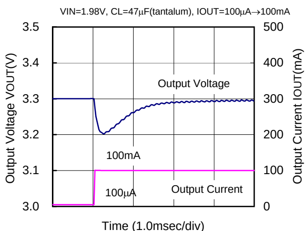
XC9103D092MR(PWM,180kHz,3.3V)
