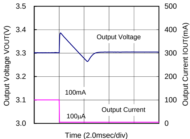
XC9103D092MR(PWM,180kHz,3.3V)
