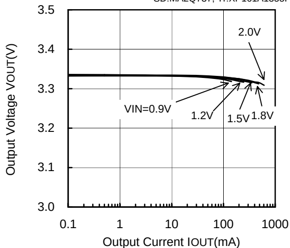
XC9104D095MR (PWM/PFM,500kHz,3.3V)
