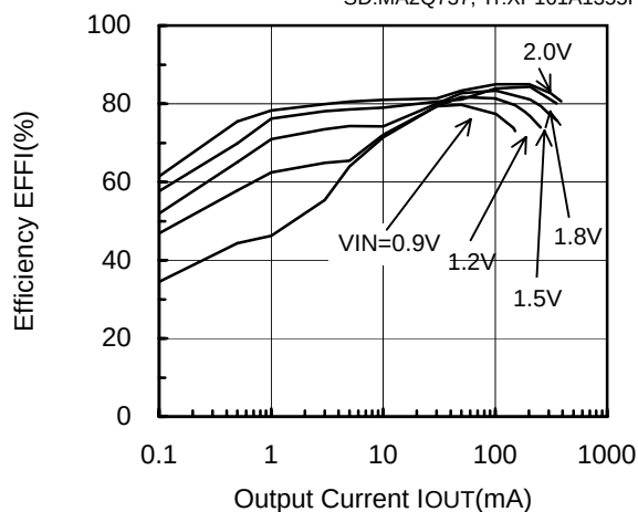
XC9104D092MR (PWM/PFM,180kHz,3.3V)
