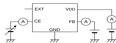
CIRCUIT ⑤
