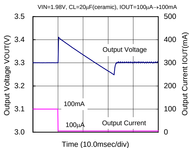
XC9104D093MR(PWM/PFM,300kHz,3.3V)
