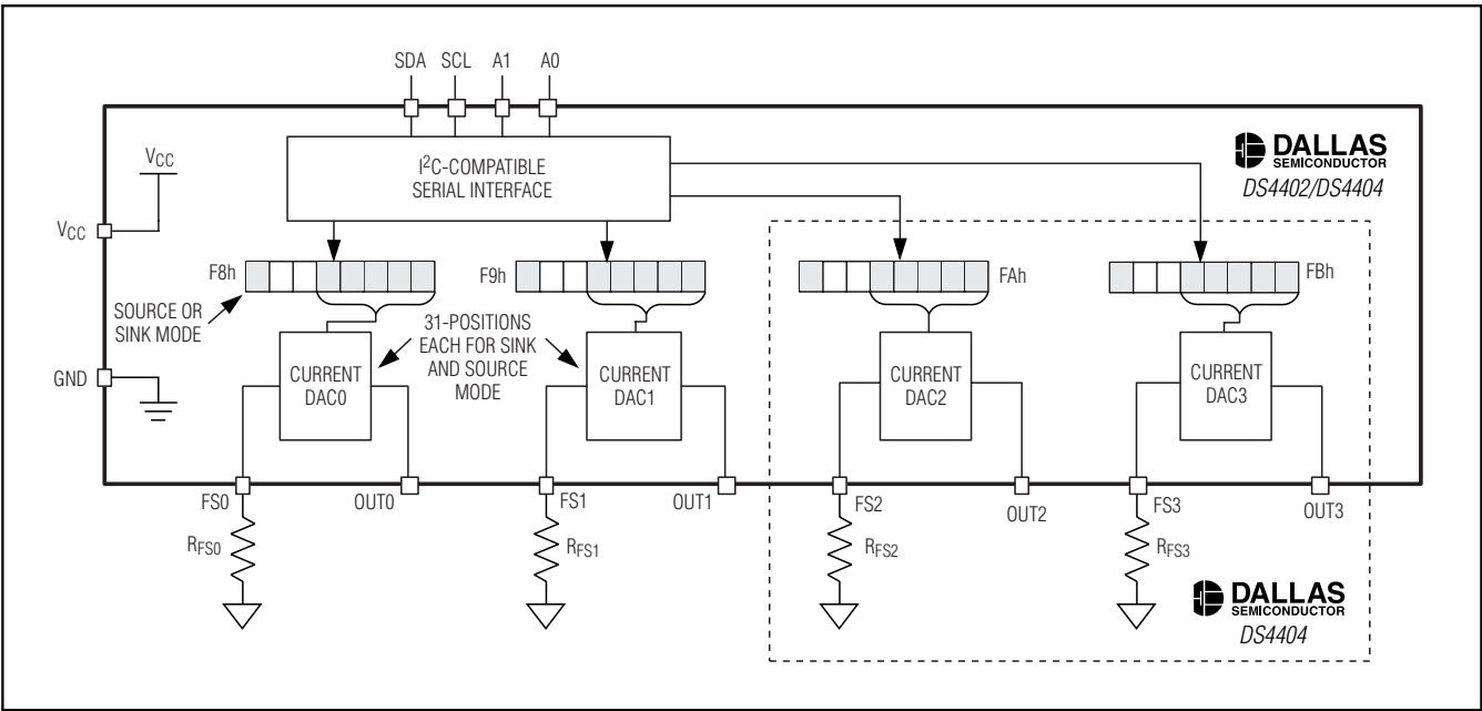
Figure 1. Functional Diagram
