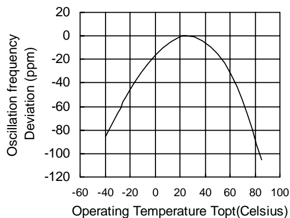
Oscillation Frequency Deviation vs. Operating Temperature ( V_{DD}=3\text{V} )
