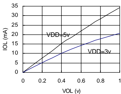
VOL vs. IOL (/INTRA, /INTRB pin) ( T_{opt}=25^{\circ}\text{C} )
