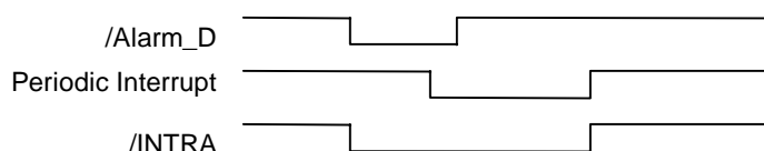
Example: Combined Output to /INTRA Pin Under Control of /Alarm_D and Periodic Interrupt
