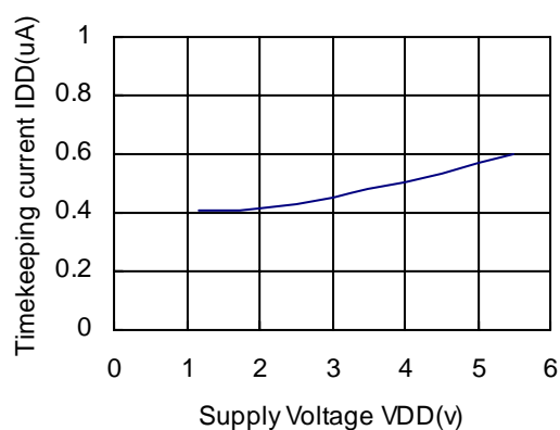
Timekeeping current vs. Supply Voltage (with no 32-kHz clock output) (Output=Open, T_{opt}=25^{\circ}\text{C} )
