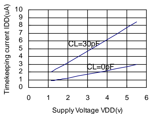
Timekeeping current vs. Supply Voltage (with 32-kHz clock output) (Output=Open, T_{opt}=25^{\circ}\text{C} )
