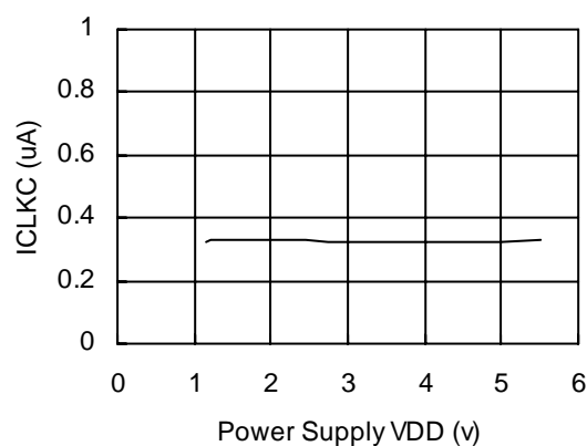
CLKC pin Input Current vs. Power Supply ( V_{IN}=V_{DD}, T_{opt}=25^{\circ}\text{C} )
