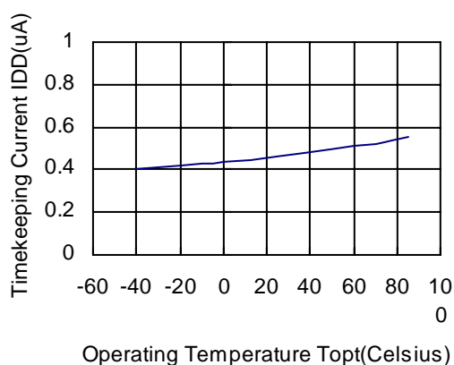
Timekeeping current vs. Operating Temperature (with no 32-kHz output) (Output=Open, V_{DD}=3\text{V} )
