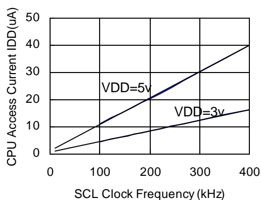
CPU Access Current vs. SCL Clock Frequency (Output=Open, T_{opt}=25^{\circ}\text{C} ) (without pull-up resistor current)
