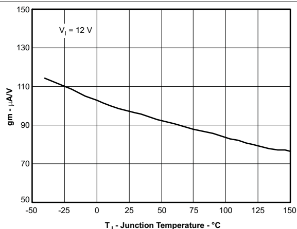
Figure 9. EA Transconductance vs Junction Temperature
