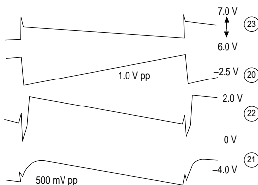
Figure 10. Vertical Waveforms
