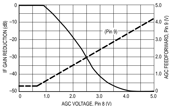
Figure 2. Monomax AGC Characteristics
