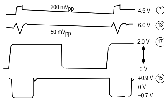
Figure 8. Horizontal Waveforms
