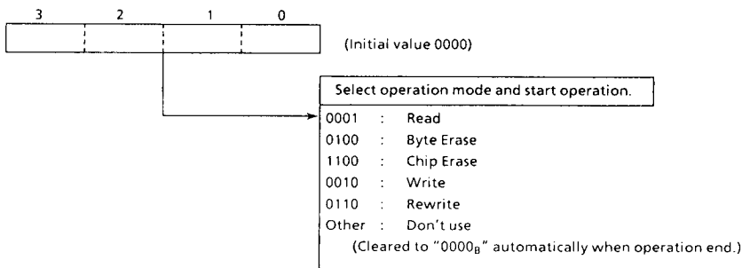
Figure 1-2. E 2 PROM command register
