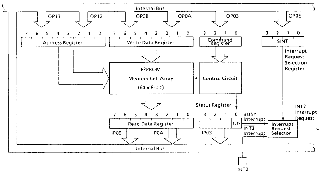
Figure 1-1. E 2 PROM
