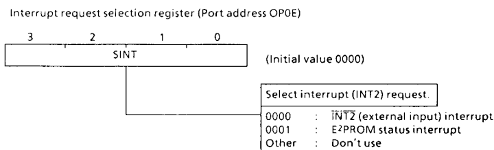
Figure 1-7. Interrupt request selection register
