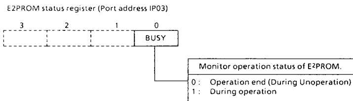
Figure 1-6. E2PROM status register
