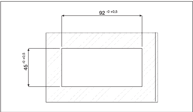
Panel cutout
