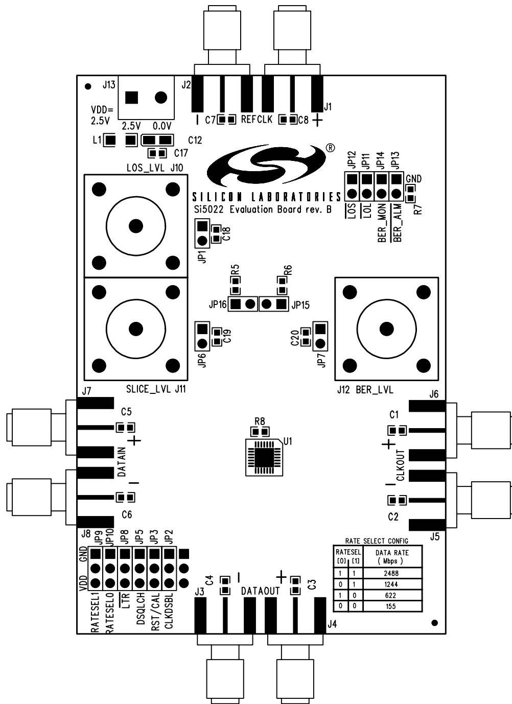
Figure 5. Si5022 Silkscreen
