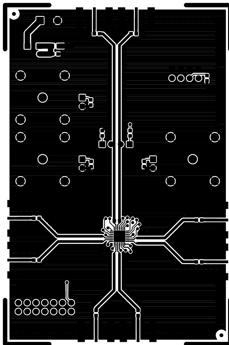
Figure 6. Si5022 Component Side
