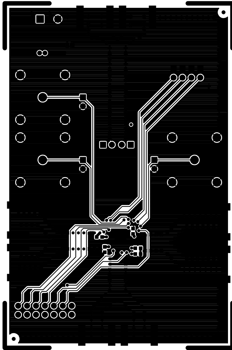
Figure 7. Si5022 Solder Side
