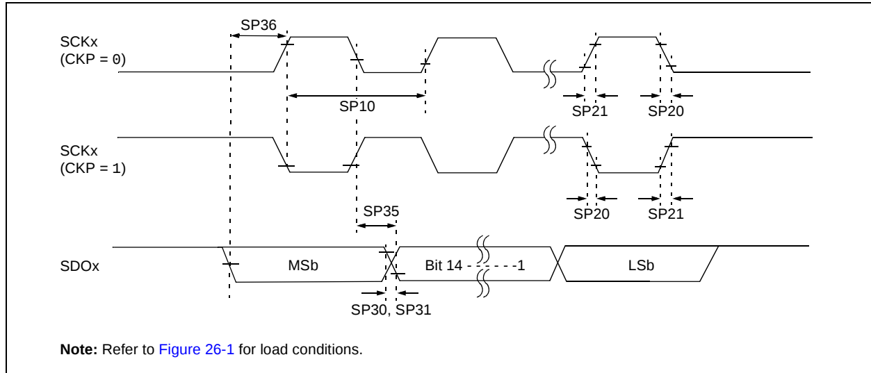
FIGURE 26-12: SPIx MASTER MODE (HALF-DUPLEX, TRANSMIT ONLY) TIMING CHARACTERISTICS FOR dsPIC33FJ16(GP/MC)10X
