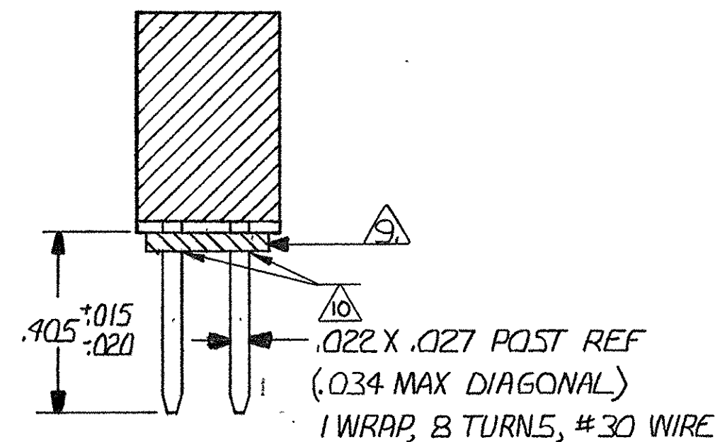
SECTION A-A RACK MOUNT (TYPE VI)
