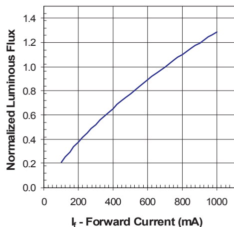
Figure 6. Relative Luminous Flux vs. Forward Current for White, Green, Cyan, Blue, and Royal Blue at T_J = 25^\circ\text{C} maintained.
