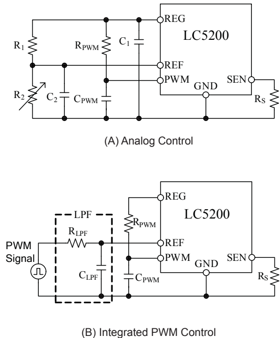
Figure 6. Dimming Application Circuits with Internal PWM Control
