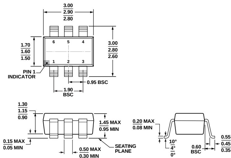
Figure 54. 6-Lead Small Outline Transistor Package [SOT-23] (RJ-6)
