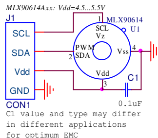
MLX90614 connection to SMBus Figure 1: Typical application schematics
