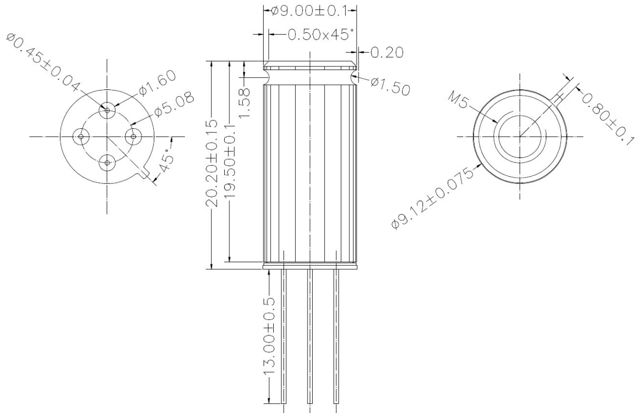
Figure 45: MLX90614xCI package
