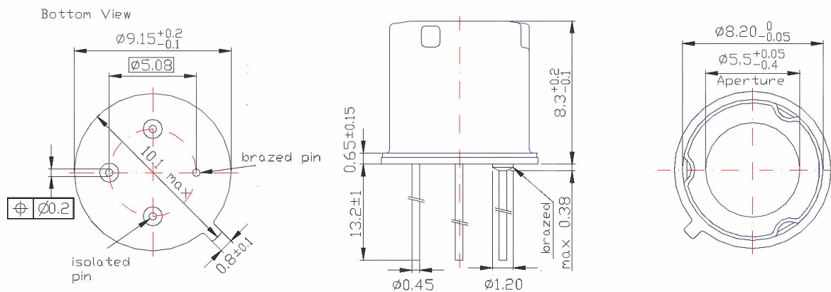
Figure 44: MLX90614xCH package
