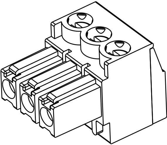
284507-3 AS SHOWN
