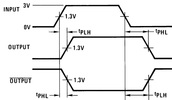
Figure 3. Propagation Delays
