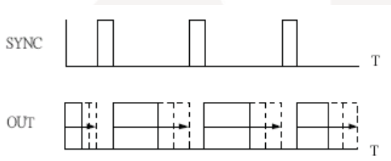
FIG.3 Synchronized Interleaving-Switching
