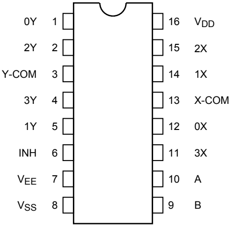
TC4052B
