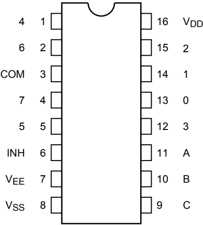
TC4051B
