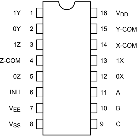
TC4053B
